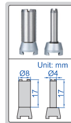
clamp (included)
