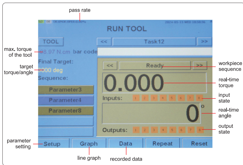
controller (included)
