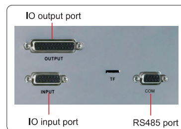
communication port (included)
