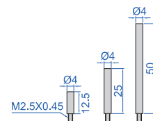
extension rods
