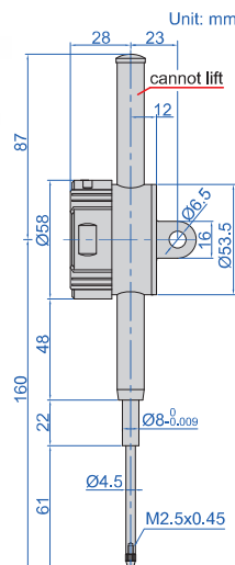
2138-50 2139-50
